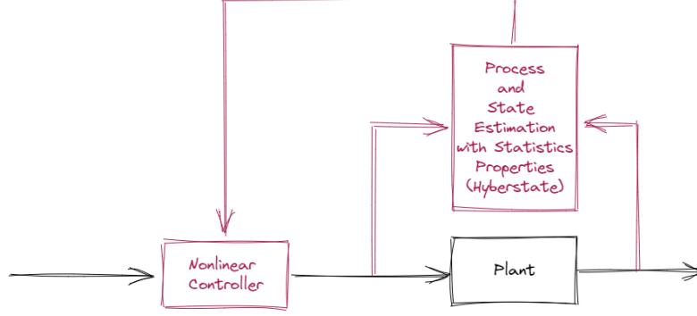
FIGURE 8.5: Dual control schema.
