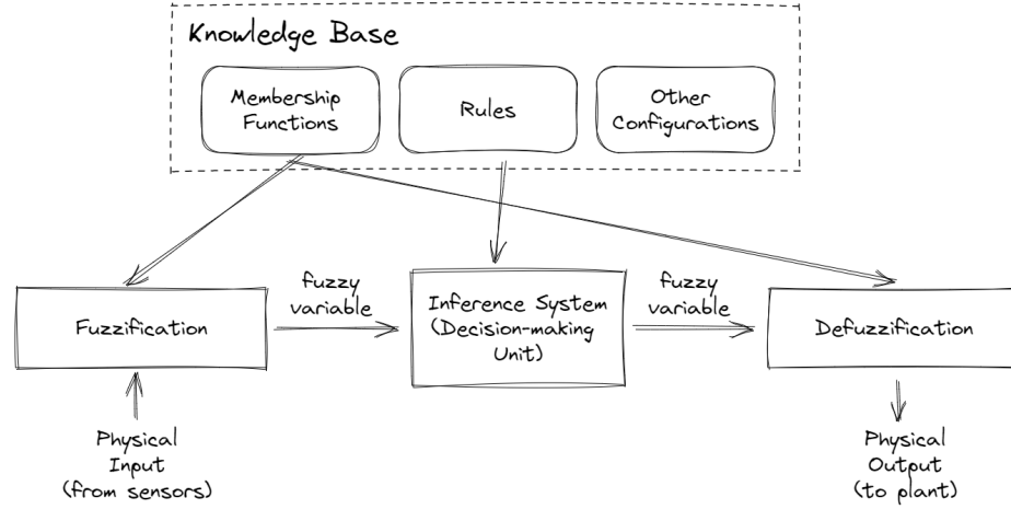
FIGURE 13.3: A simple schema for a fuzzy control system.
