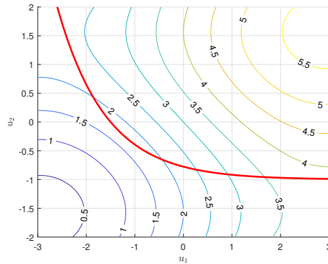
FIGURE 5.1: Static optimization with equality constraint demonstration.
