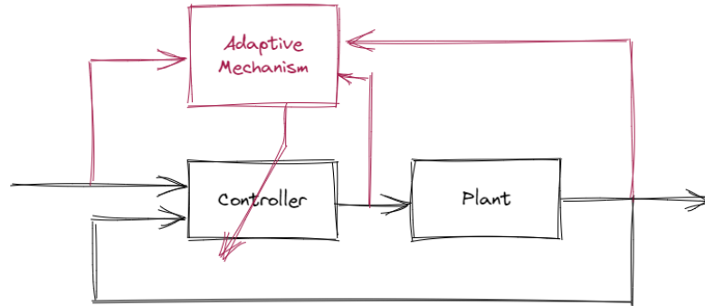
FIGURE 8.1: Adaptive control system general schema.
