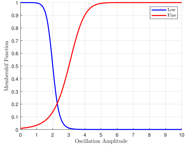
FIGURE 13.5: Membership functions for 2 fuzzy sets “low” and “fine” defined on input signal oscillation amplitude.
