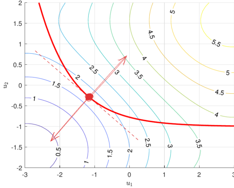
FIGURE 5.2: Graphical explanation to (5.7).
