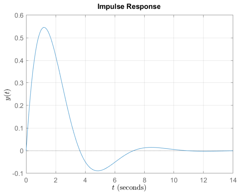
FIGURE 8.6: LTI system impulse response demonstration.
