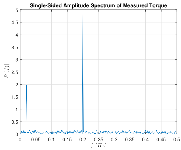
FIGURE 13.8: Measured torque single-sided amplitude spectrum.
